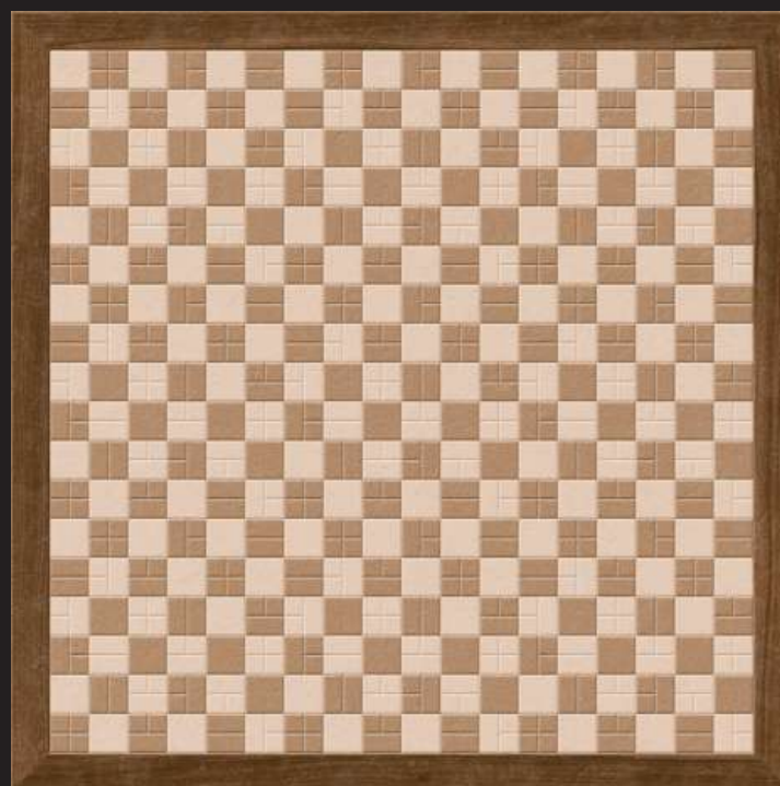
TALC-114
