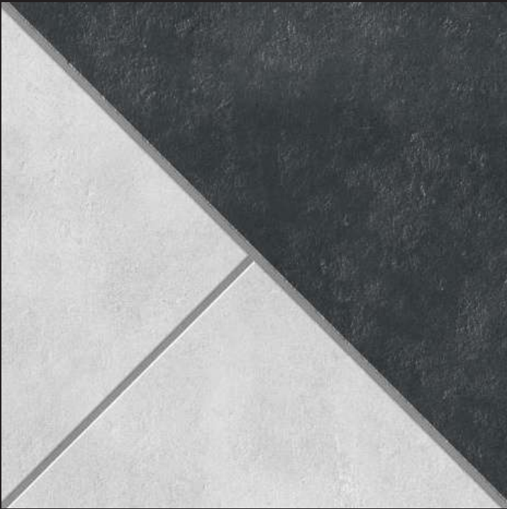
FLUORITE-111
