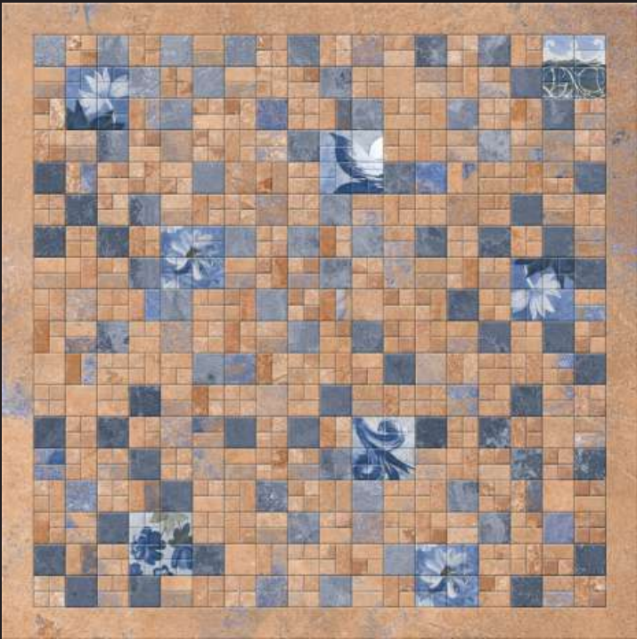
TALC-101
