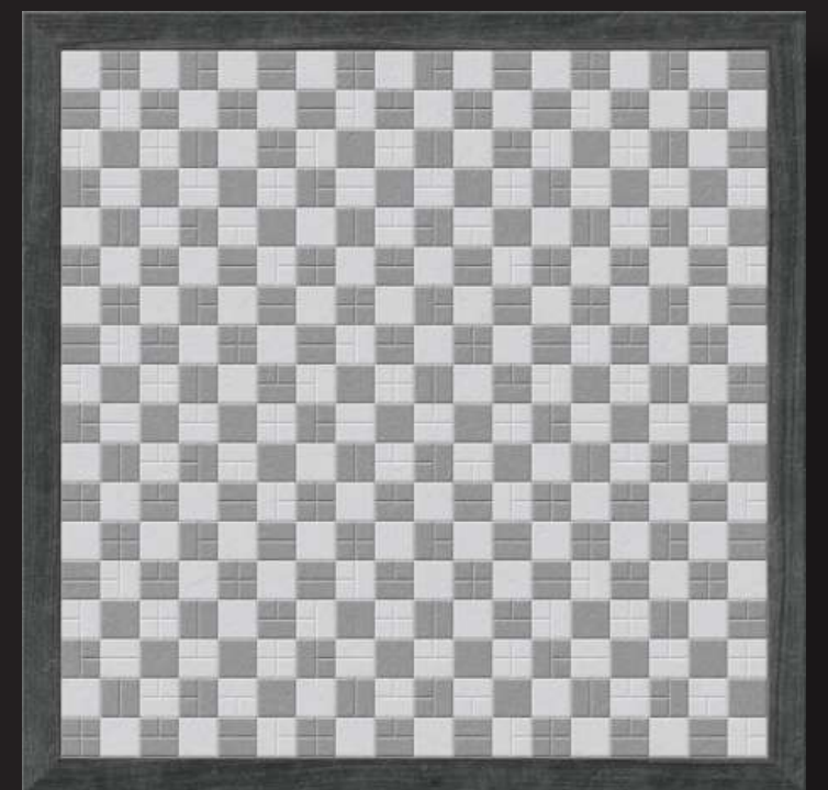
TALC-115
