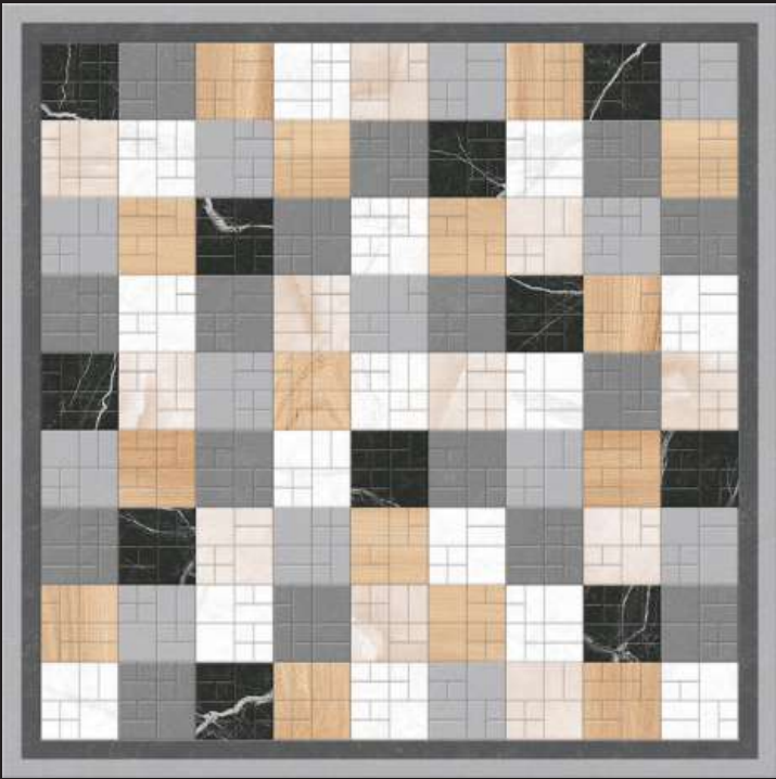
TALC-103
