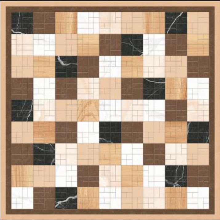
TALC-104
