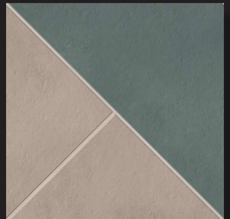
FLUORITE-132
