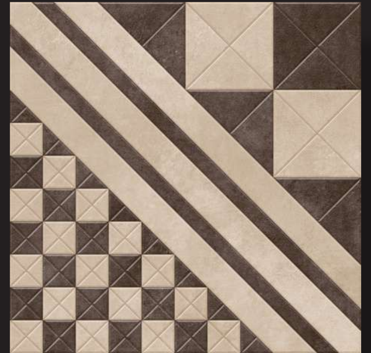
AGATE-122
