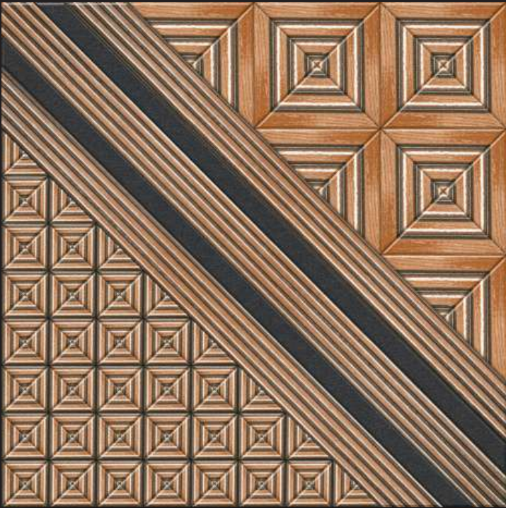
AGATE-111
