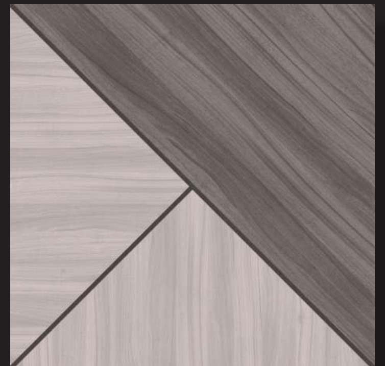
FLUORITE-124
