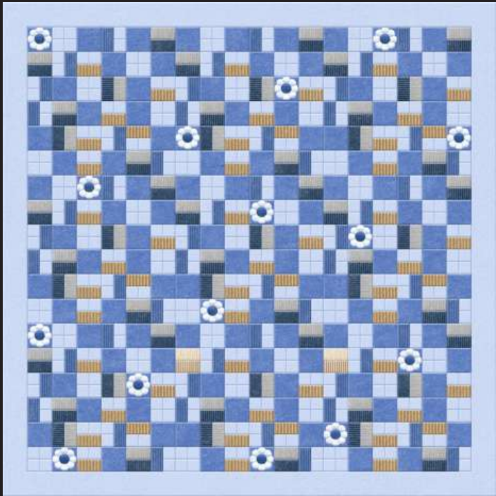
TALC-110
