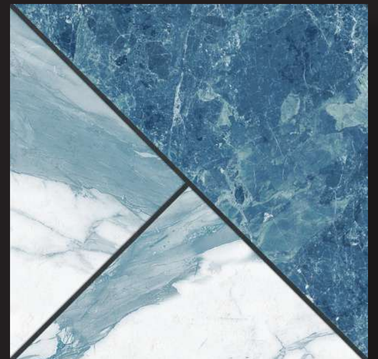
FLUORITE-116
