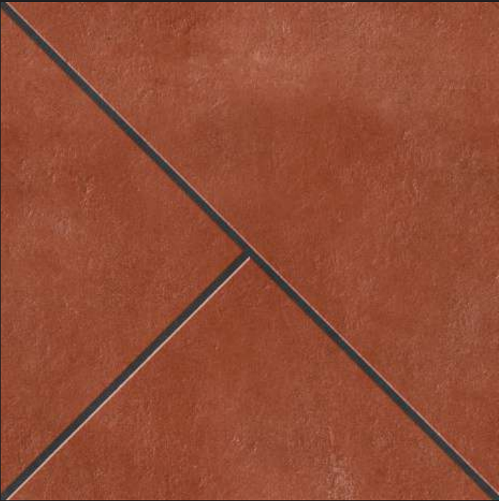
FLUORITE-112
