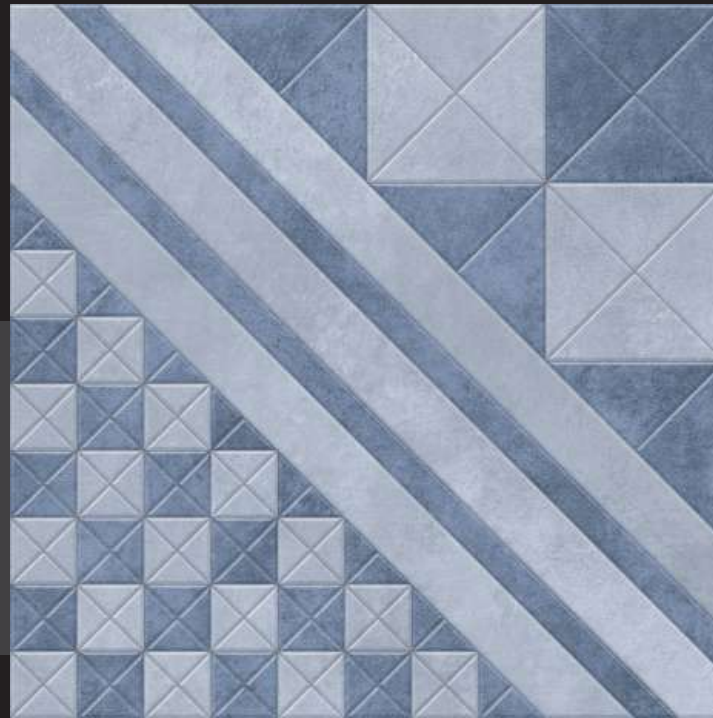
AGATE-121
