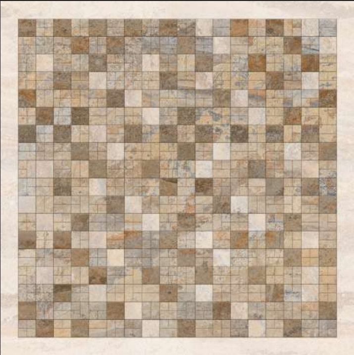
TALC-118
