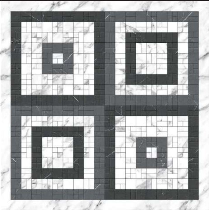
TALC-102
