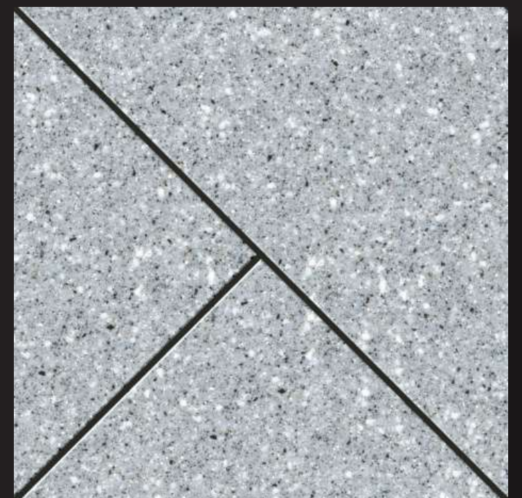
FLUORITE-108
