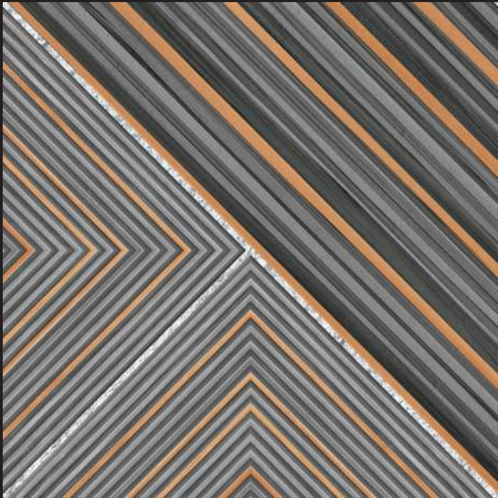
FLUORITE-118
