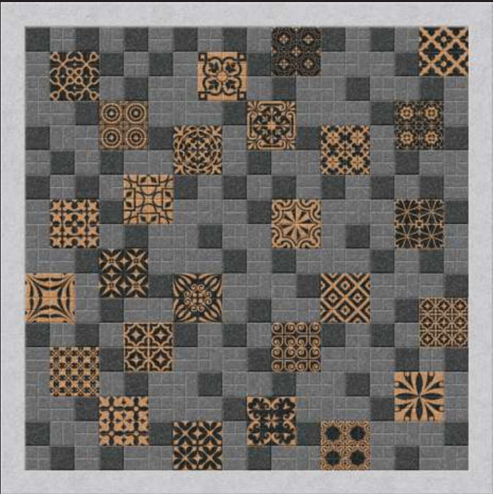
TALC-117
